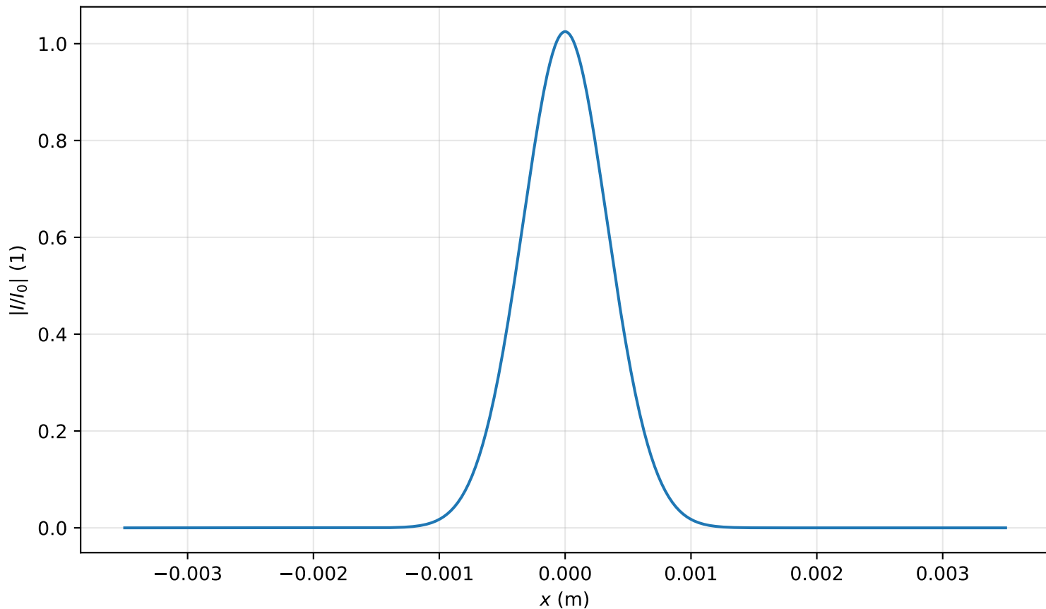
Intensity profile I(x, y = 0, z = 0.239m)/I_0 , P_{in}=0.7P_{cr} , artificial time
